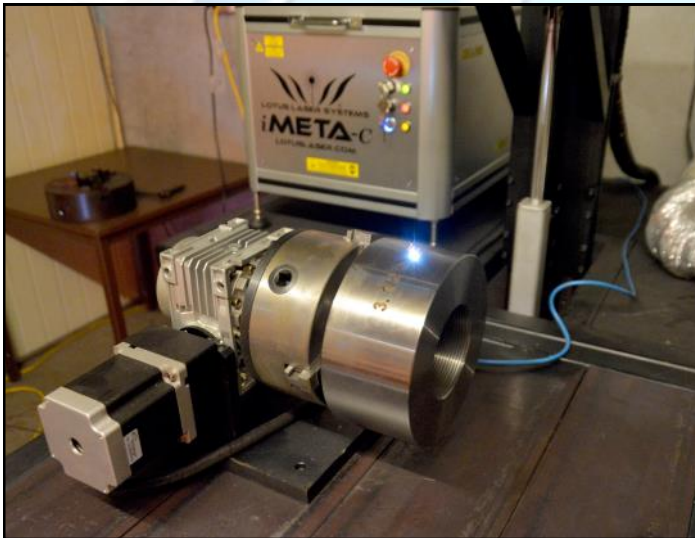
Technofast Industries' laser has a fourth axis rotation, as shown above.
